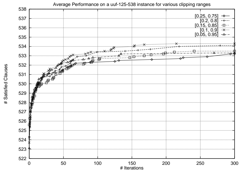
Fig. 4. Average Performance over ten runs for each clipping range
