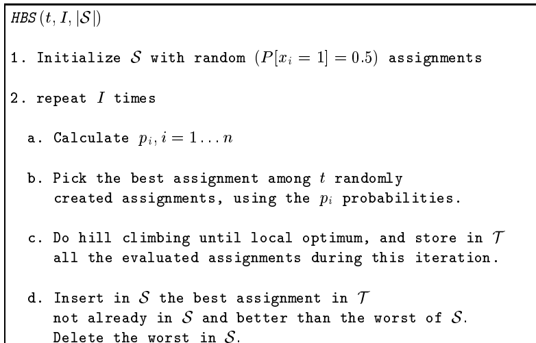
Fig. 1. The complete HBS algorithm
